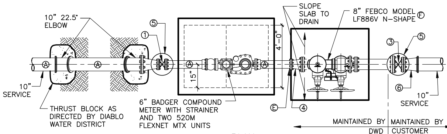
PLAN NTS
