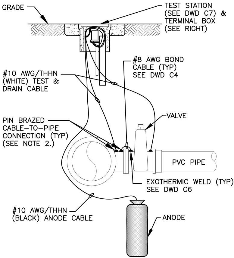
PROFILE
