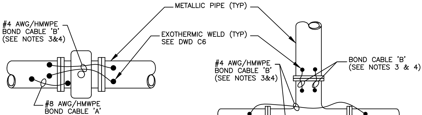
VALVE
